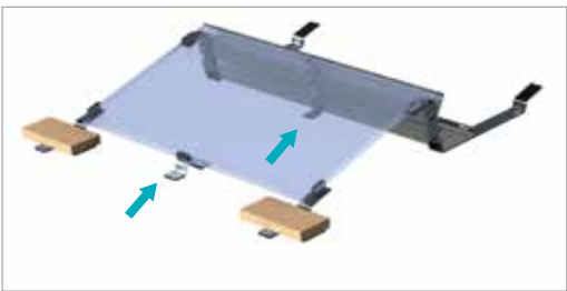
4,400 Pa (test load) – with “Alpine” support
